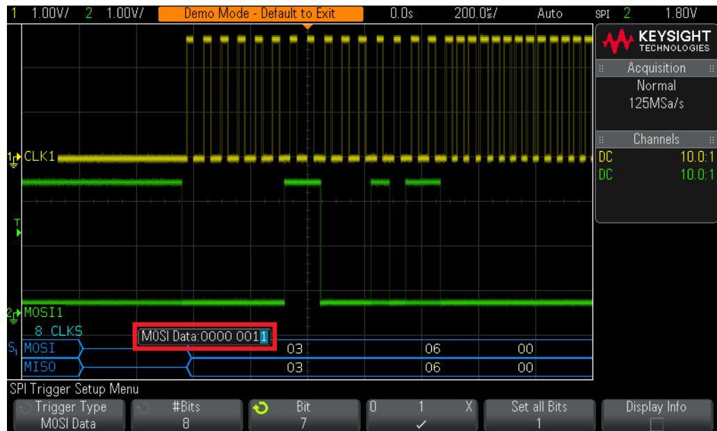
Figure 40 Triggering on MOSI data = 03 HEX .
